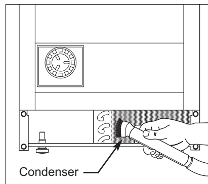
Figure 4-1. Condenser Cleaning
