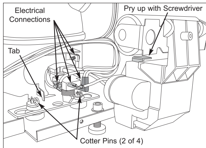
Figure 5-34. Compressor Removal
