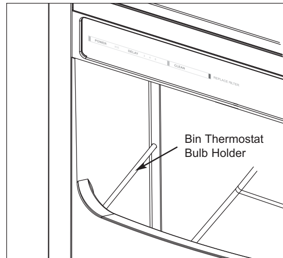
Figure 3-13. Ice Bin Storage Level
