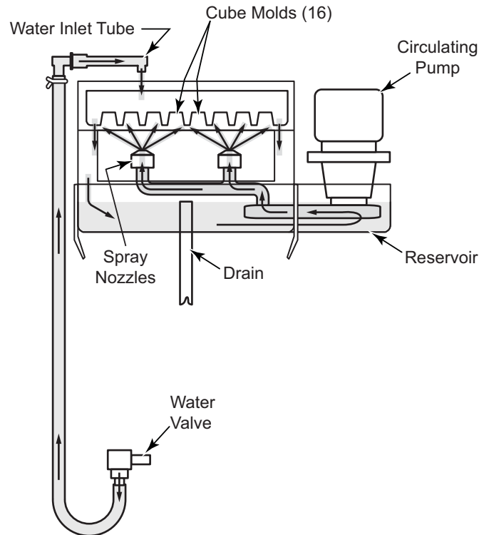
Figure 3-3. Water System (Beginning of Ice Making Cycle)
