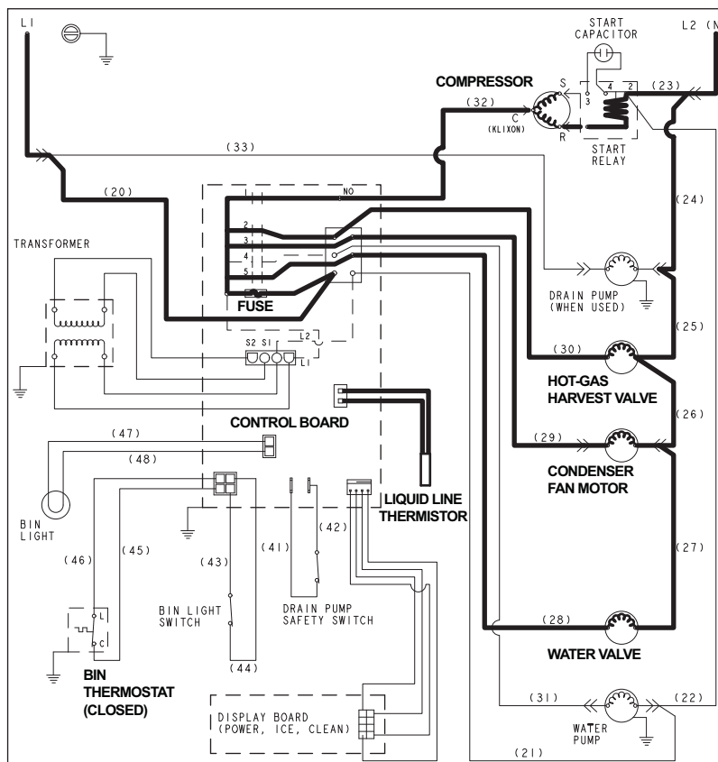
Figure 3-9. Wire Diagram - Harvest Cycle
