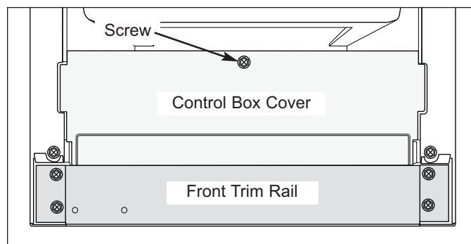
Figure 5-15. Control Box Cover Removal
