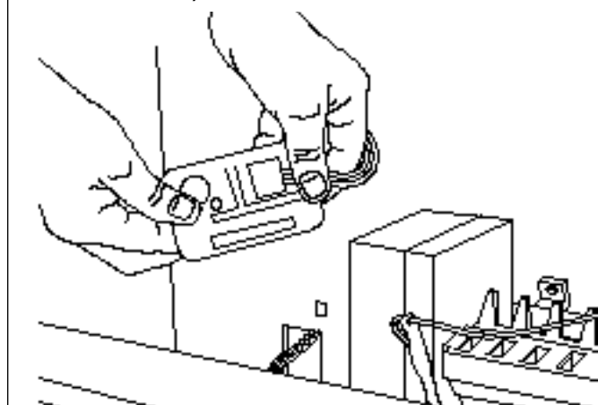
Figure 2-15. Thermistor Location
