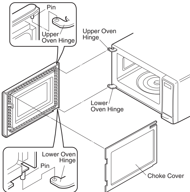
Figure C-5. Door Replacement
