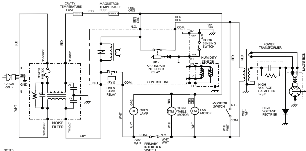
Figure O-2 Oven Schematic - Cooking Condition
