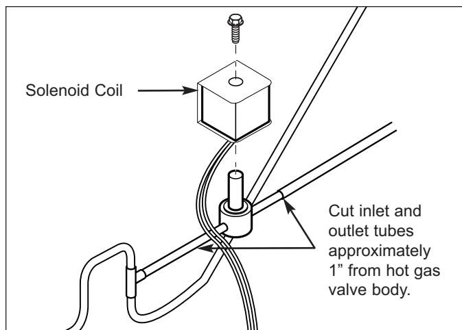
Figure 5-32. Hot Gas Valve Removal
