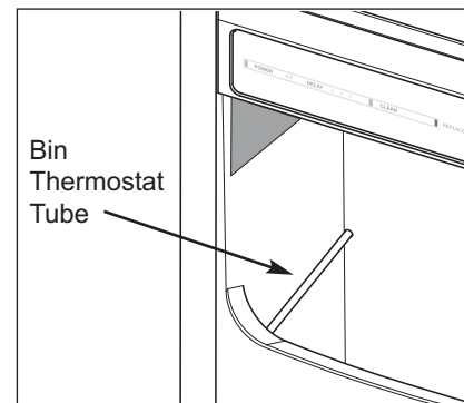
Figure 4-20. Bin Thermostat Tube Location
