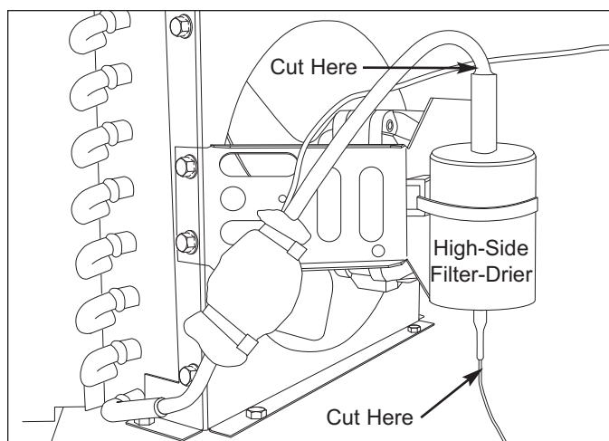
Figure 5-33. High-Side Filter-Drier Removal
